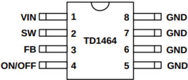
Figure1 Pin Configuration of TD1464(Top View)
