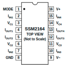
PIN CONFIGURATION 16-Lead Epoxy DIP and SOIC
